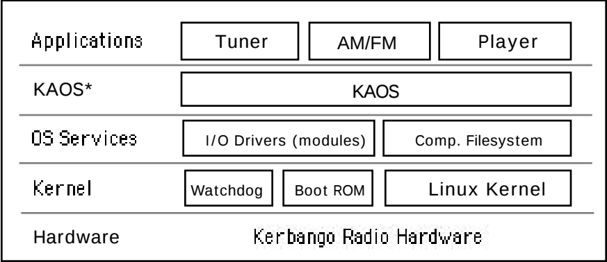
Kerbango Radio Software Architecture
