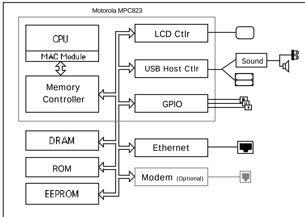
Kerbango Internet Radio Block Diagram
